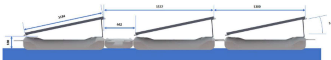
Figure 4 – Profil de la centrale flottante (Source : Laketricity)
